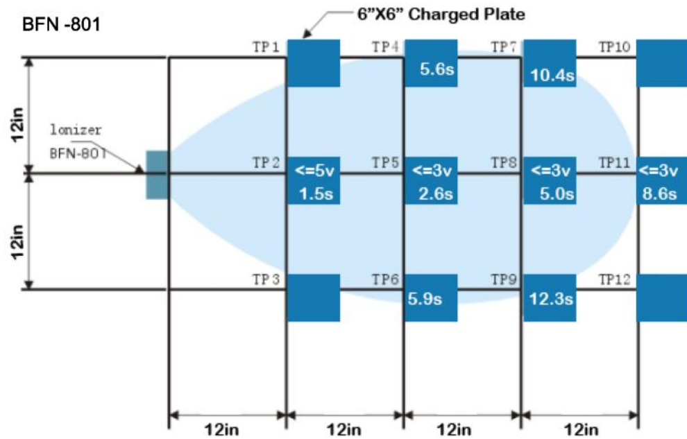
Data chart of delay time and ion balance, 1000v to 100v
